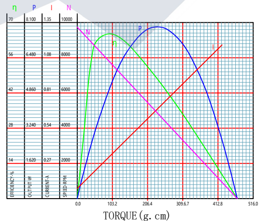
BL2838I-V3 Performance curves
