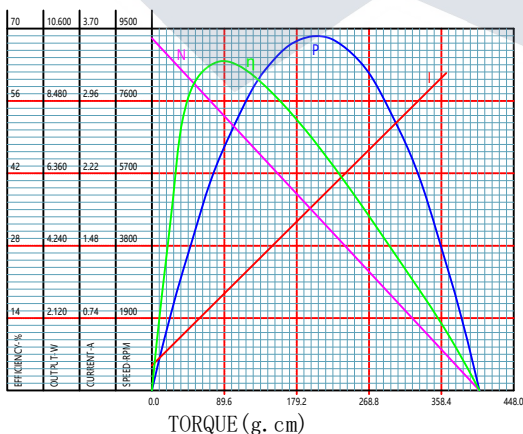
BL2838I-V2 Performance curves
